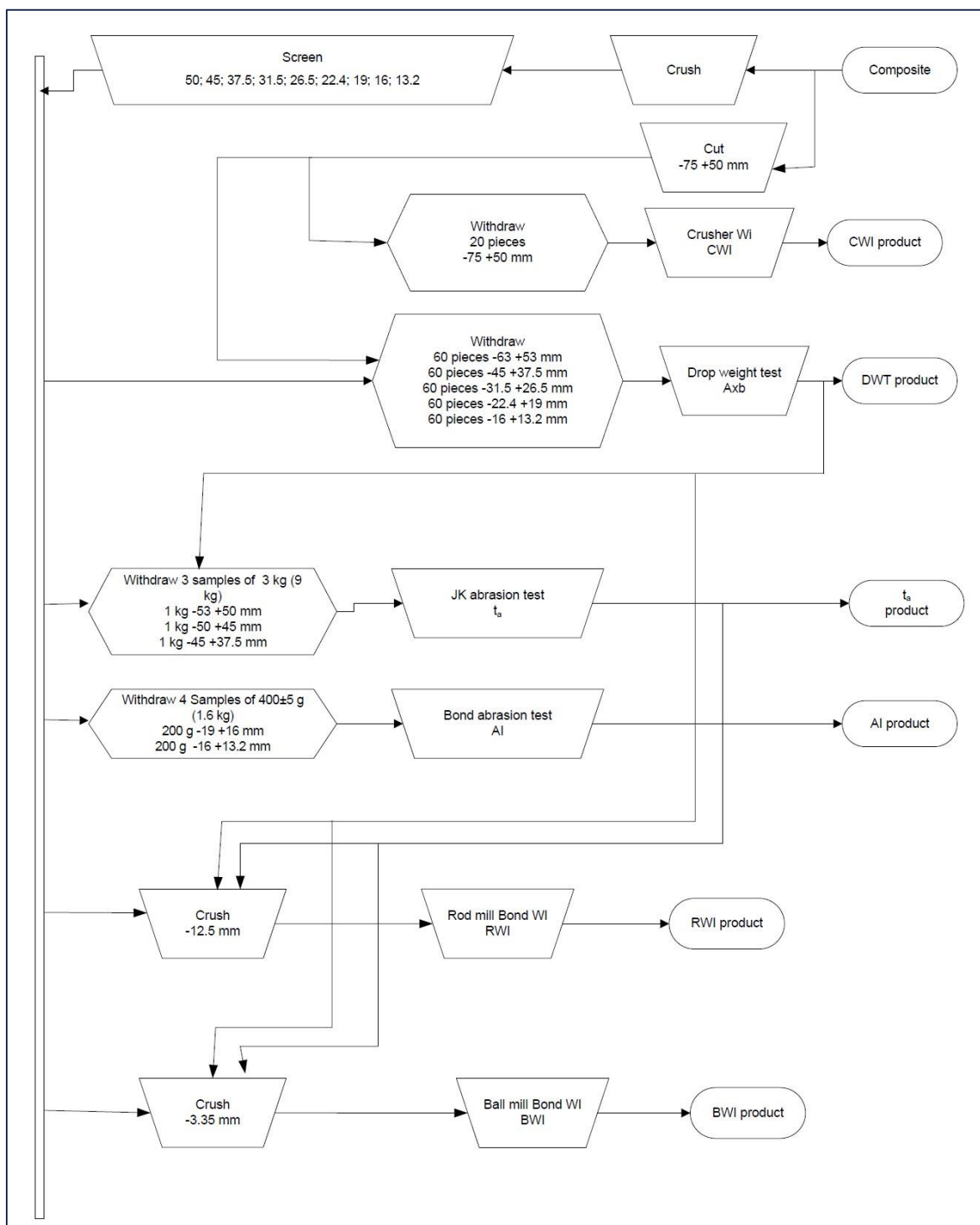
Figure 13-2: COREM comminution testwork protocol
